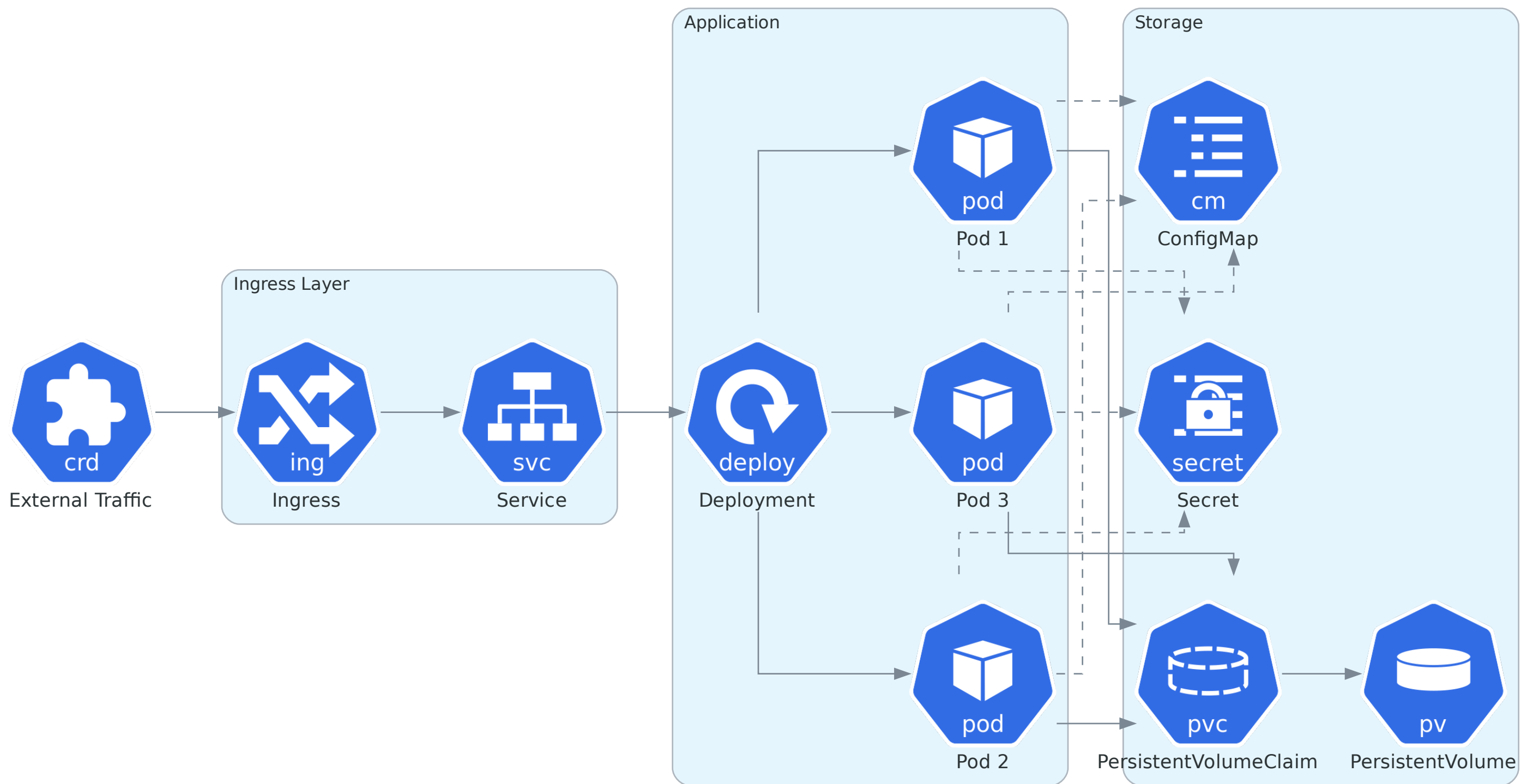
Kubernetes Deployment
